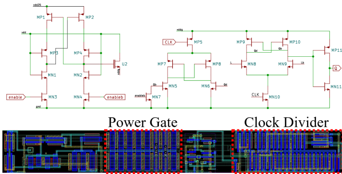
Figure 7: Schematic (Top) and Layout (Bottom) of the clock gate/divider.
