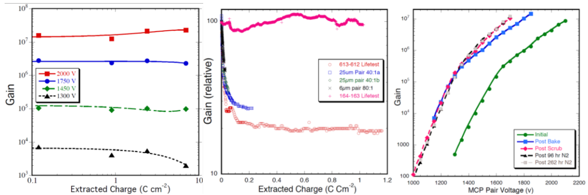
Figure 3. (Left) Gain is high and stable vs. extracted charge. Plot is of MCP gain at several fixed voltages during a “burn-in” test extracting 7 C/cm 2 at ~3 µA output current for a pair of 33 mm, 60:1 L/D, 20 µm pore ALD MCPs [8]. (Center) Conventional MCPs require an extensive “burn-in” to achieve a stable gain. Little or no burn-in is required for Incom MCPs (magenta trace) [9]. (Right) Gain of a pair of 33mm 20 µm pore, 60:1 L/D, MgO-ALD MCPs during preconditioning steps. Gain increases 10x after initial bake, and does not drop after storage for ten days in N 2 . No reconditioning is needed after breaking vacuum [6].
