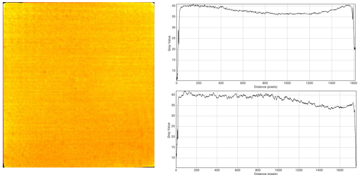
Figure 4. (Left) Gain map image for a pair of 20 µm pore, 60:1 L/D, ALD borosilicate MCPs, 950 V per MCP, 184 nm UV illumination. (Right) Gain vs. position along horizontal (top) and vertical (bottom) traverses of the plate. Gain is uniform within ~15% across the full 20 x 20 cm area [10].
